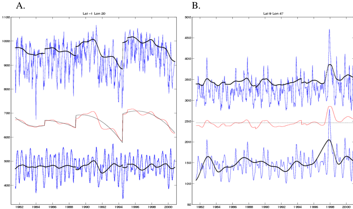
Figure 3. EMD decomposition and removal of SZA-correlated trends. A. Before satellite drift correction (series at top), trend removed (middle) and resulting series (bottom). B. Example of a pixel that is not corrected due to lack of correlation with the SZA trends.
