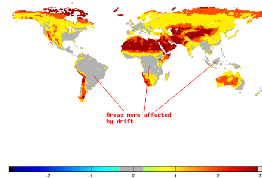
Figure 4. Regions where satellite drift has an important contribution to the signal.
